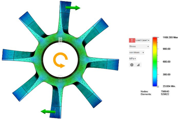
Figure 14: Fusion360 Stress simulation of screw with centrifugal and lateral loads.
