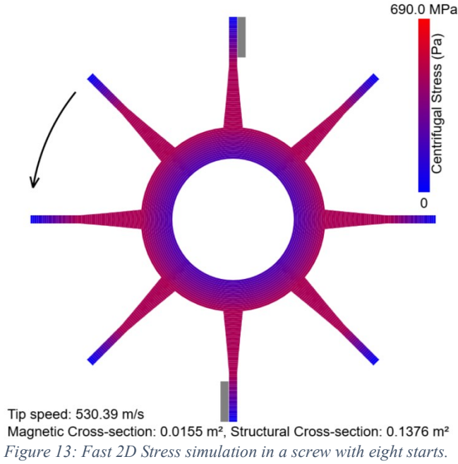
Figure 13: Fast 2D Stress simulation in a screw with eight starts.
